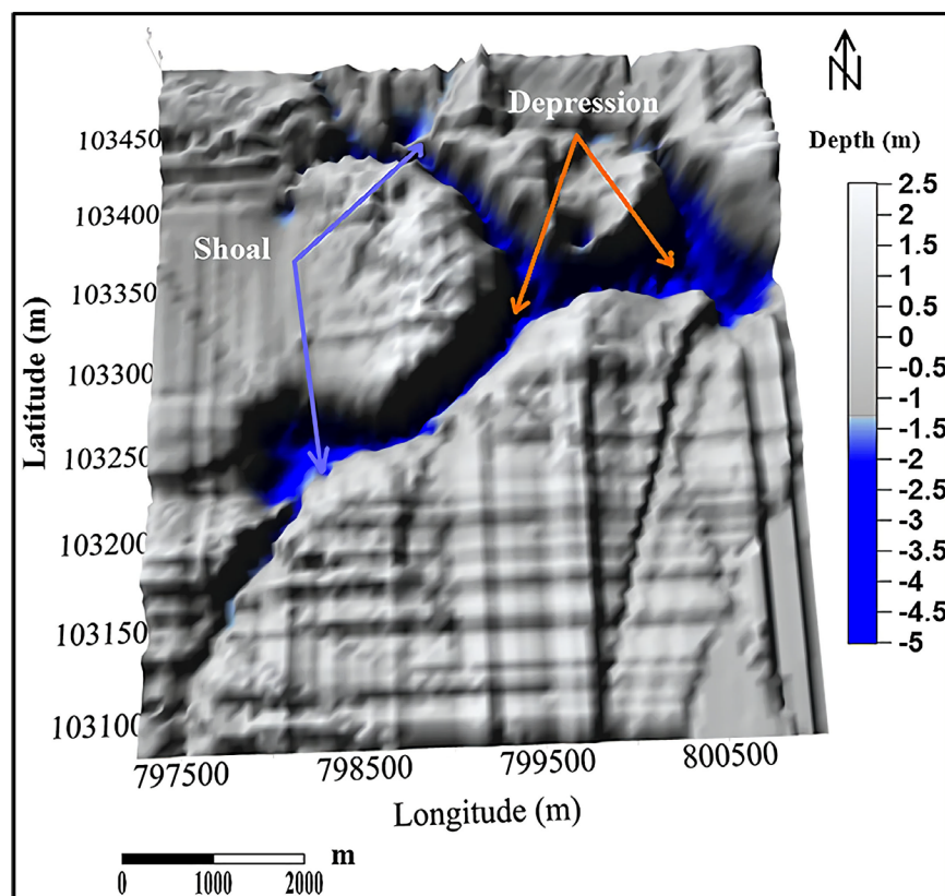
Figure 5. Digital elevation model of the lake bottom of lake Nafoun.
