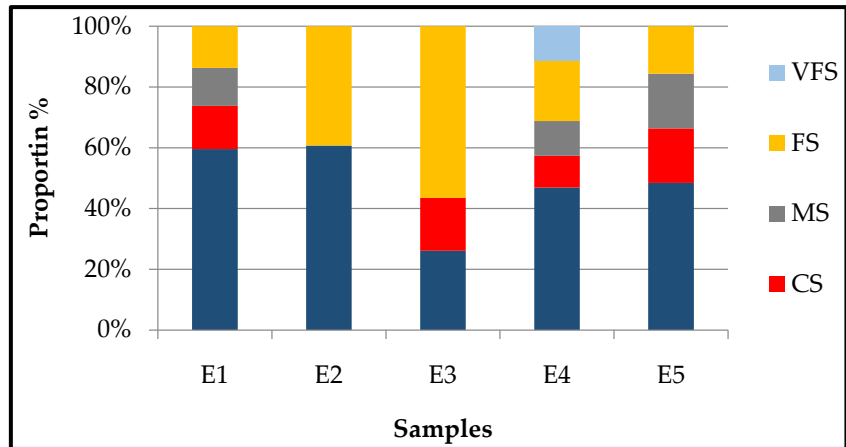
Figure 3. Percentage of the grain size fractions of the sands of the Nafoun dam (VCS: Very Coarse Sand; CS: Coarse Sand; MS: Medium Sand; FS: Fine Sand; VFS: Very Fine Sand).
