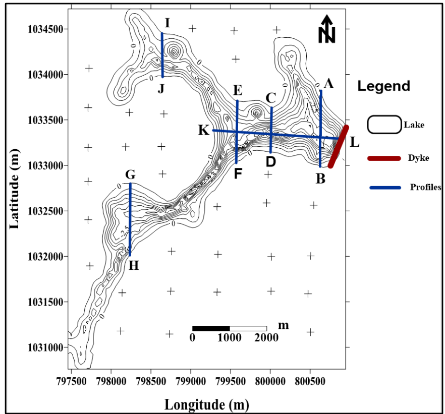
Figure 6. Bathymetric profiles at various points in Lake Nafoun.
