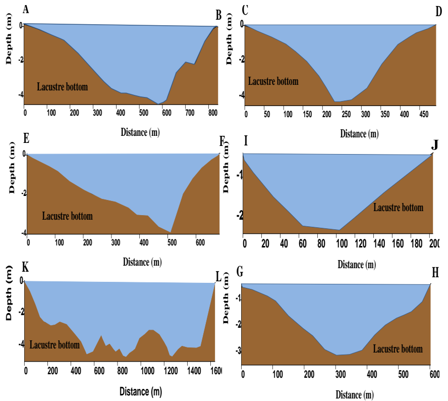
Figure 7. Bathymetric profiles of the Nafoun main channel.
