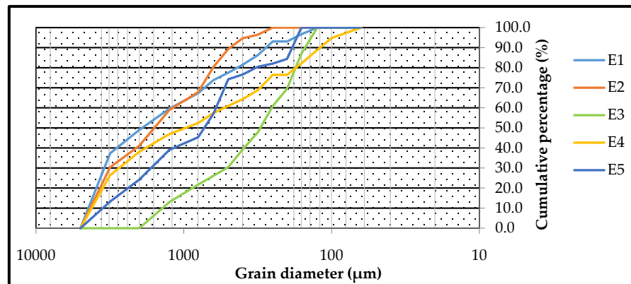
Figure 2. Particle size distribution curves of Nafoun lake sands.
